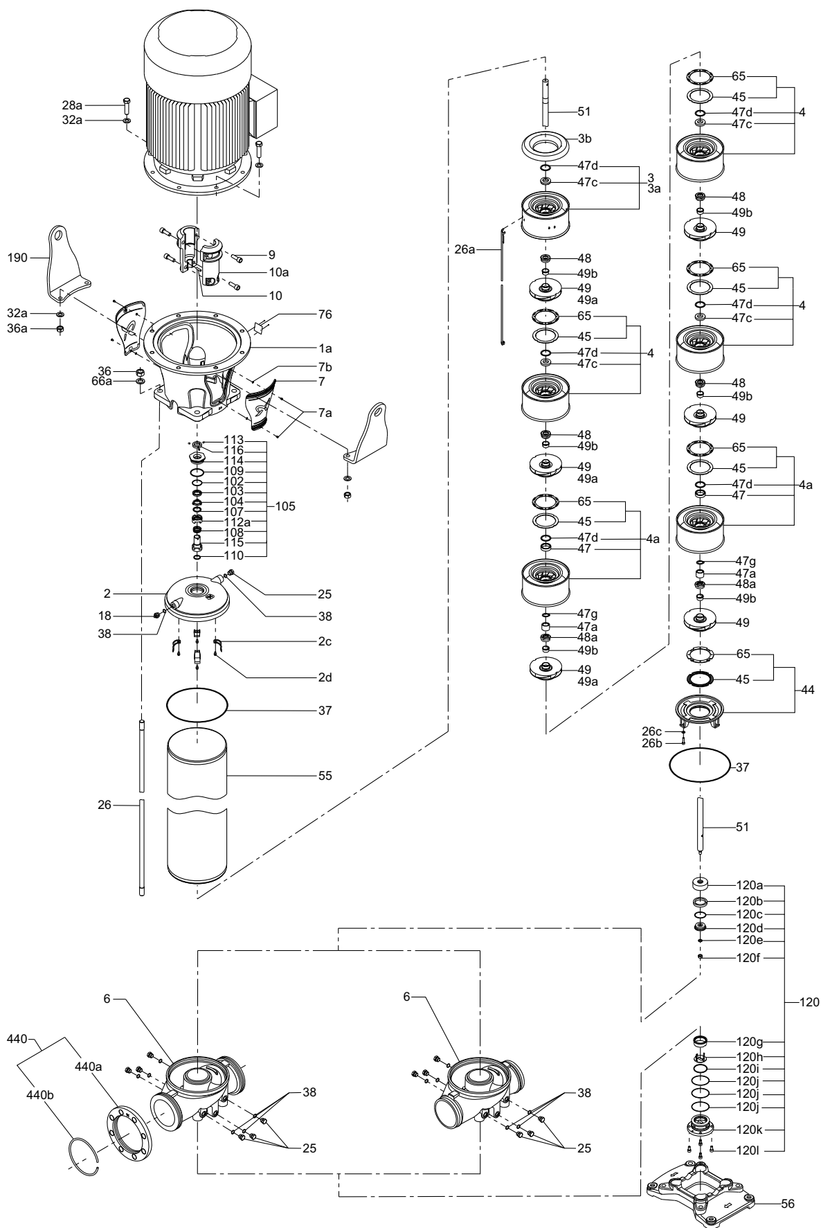
Fig. 3 Exploded view of CR, CRN pump with Ø28 or Ø36 shaft and with thrust-handling device
