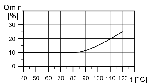
Fig. 61 Minimum flow rate
