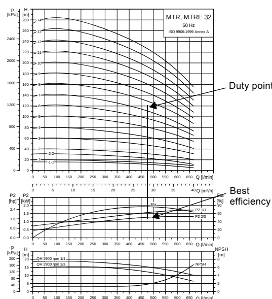
Fig. 49 Example of an MTR pump's duty point
