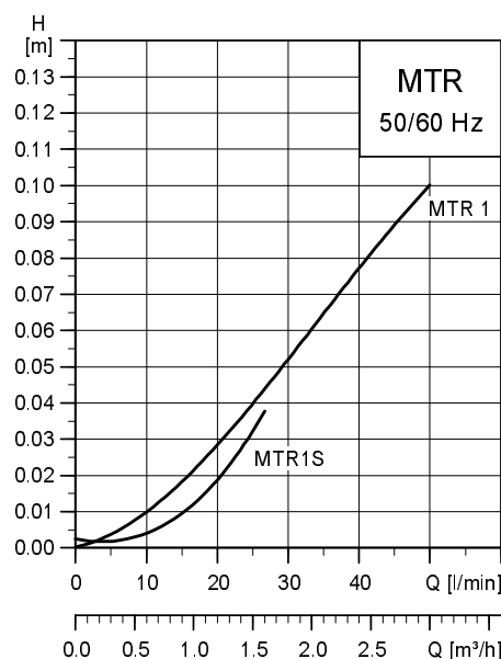
Fig. 54 Pressure losses of pumped liquid passing through an empty chamber for MTR 1s and MTR 1 pumps
