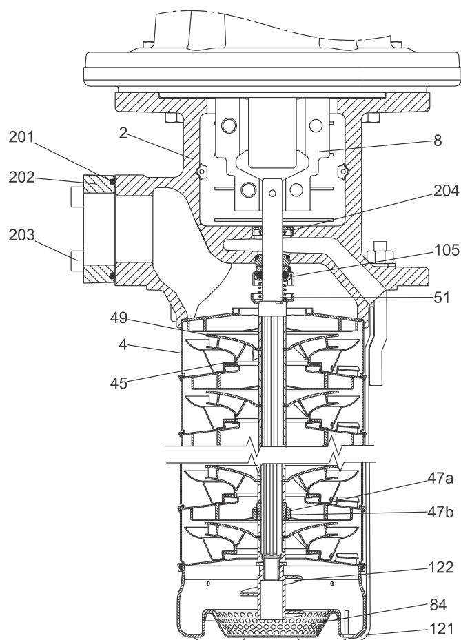
Fig. 21 MTR, MTRE 10, 15 and 20 with drainage back to tank
