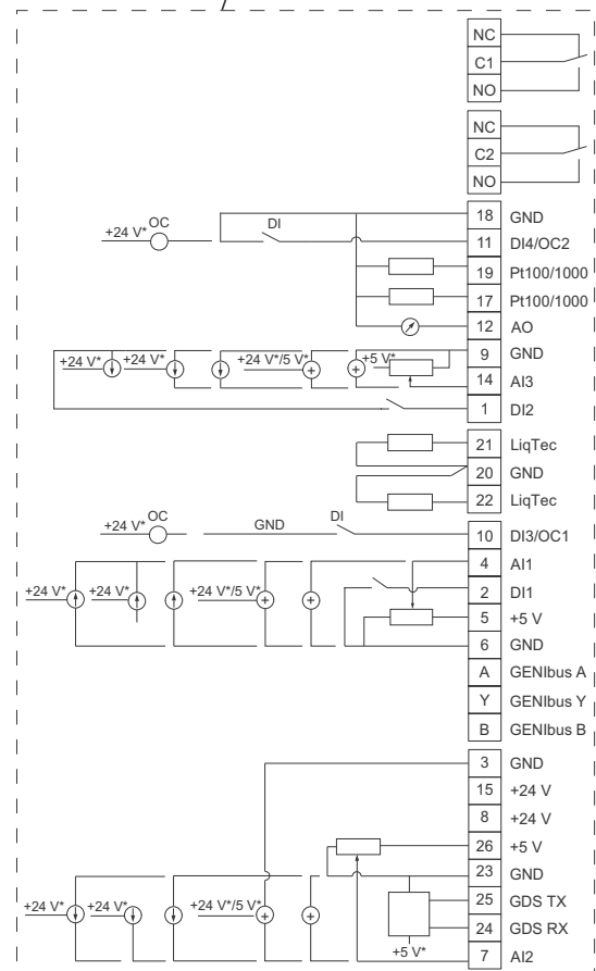
Fig. 16 Connection terminals, FM 300 functional module
