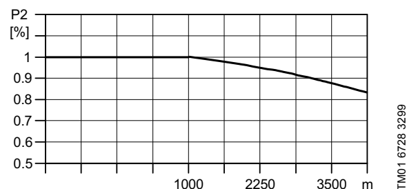
Fig. 8 Derating of motor output (P2) in relation to altitude above sea level
