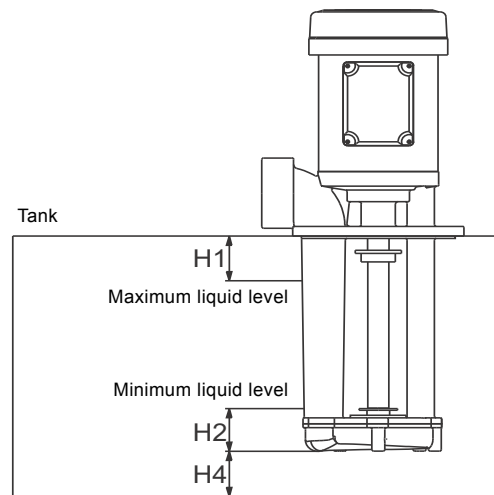
Fig. 41 MTA with bottom suction
