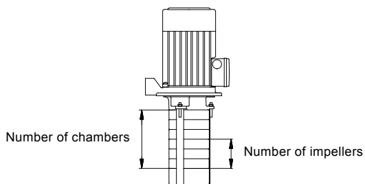
Fig. 28 MTH pump
