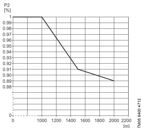
Fig. 7 Derating of motor output (P2) in relation to altitude above sea level
