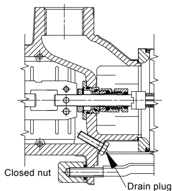
Fig. 74 Horizontal installation
