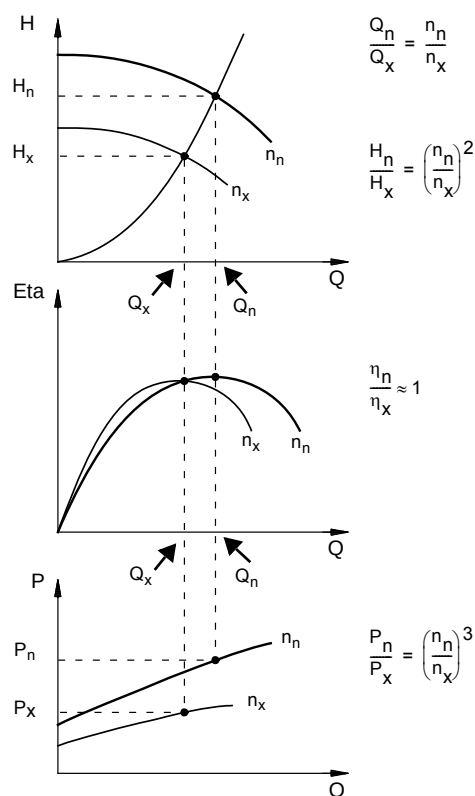
Fig. 53 Affinity equations
