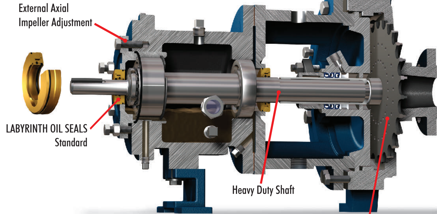
Open/Non-Clogging Radial Vane Impeller with Balance Holes
